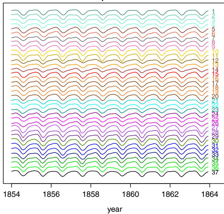
Laplacian-2
