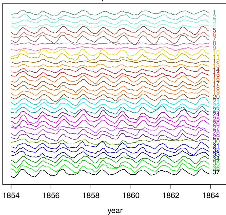
Laplacian-3
