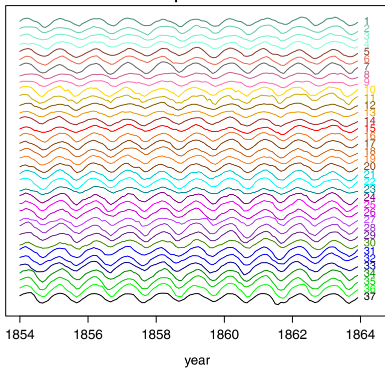
Laplacian-4
