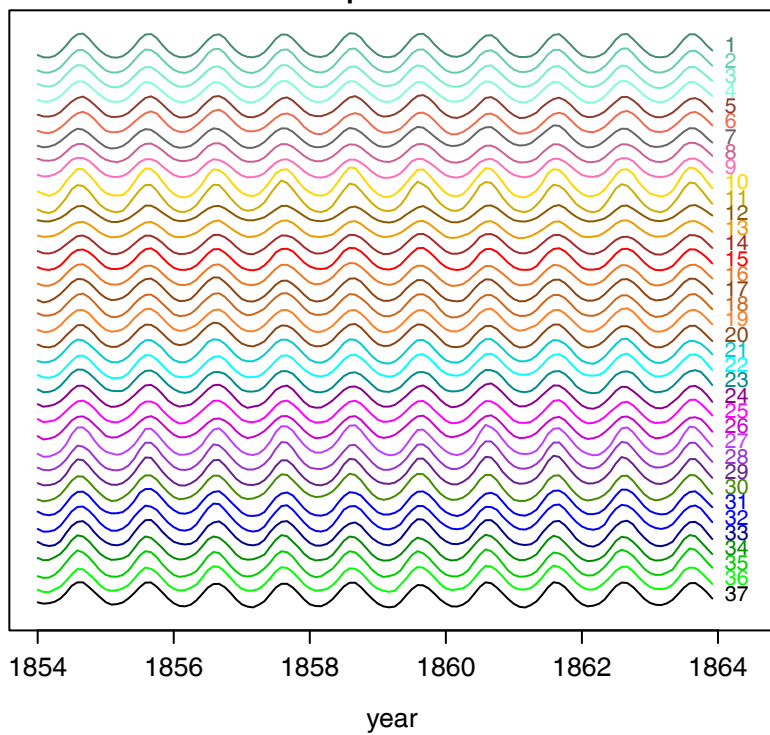
Laplacian-1
