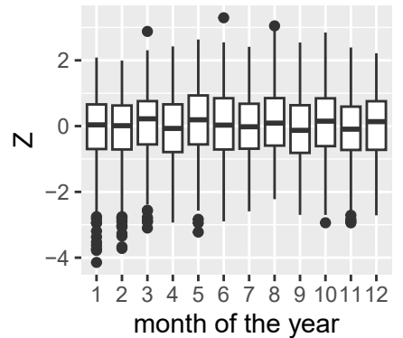
Boxplot of Z(s, t)
