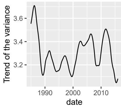
T_\sigma(s, t)
