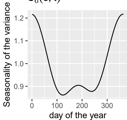
S_\sigma(s, t)
