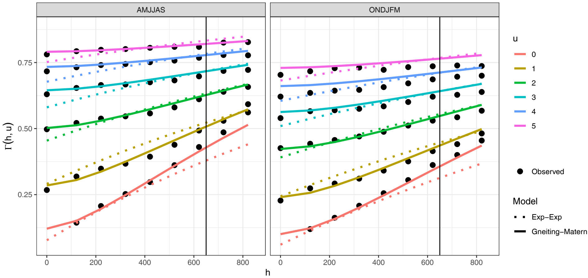
Empirical variogram VS fitted variograms
