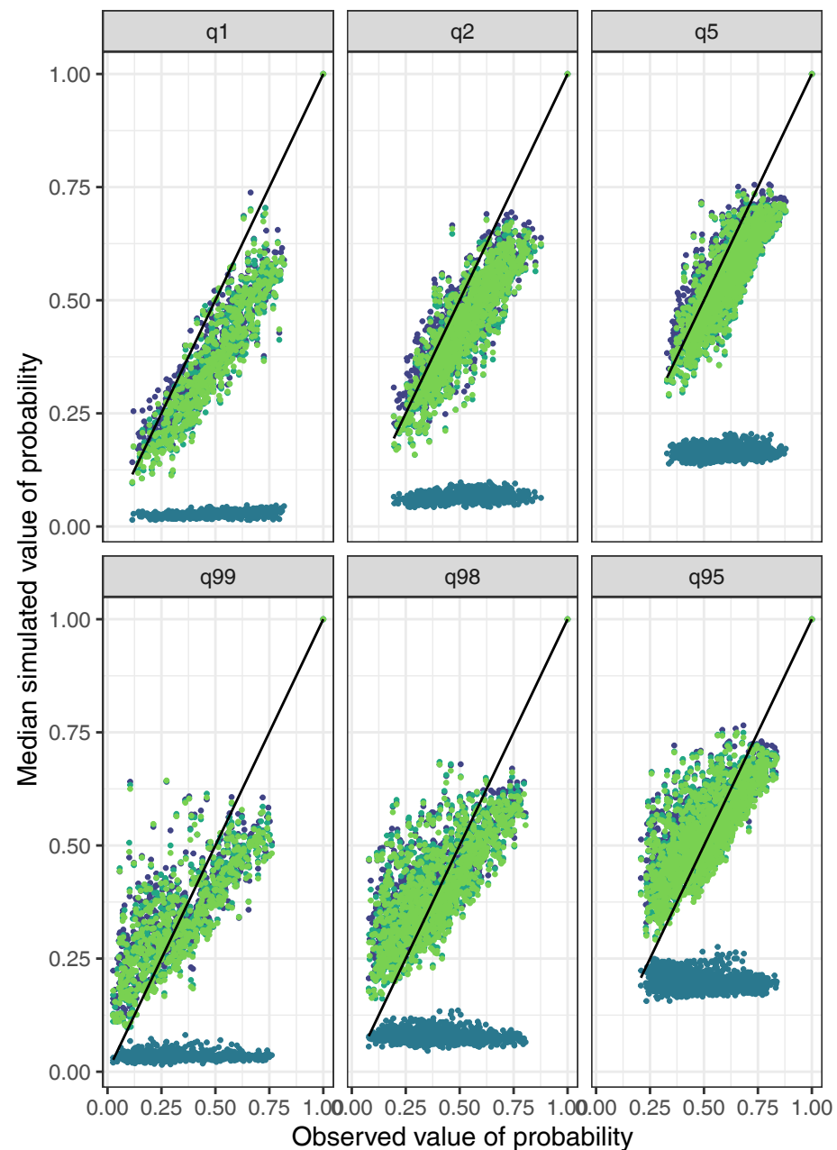
Probability of conditional threshold exceedance
