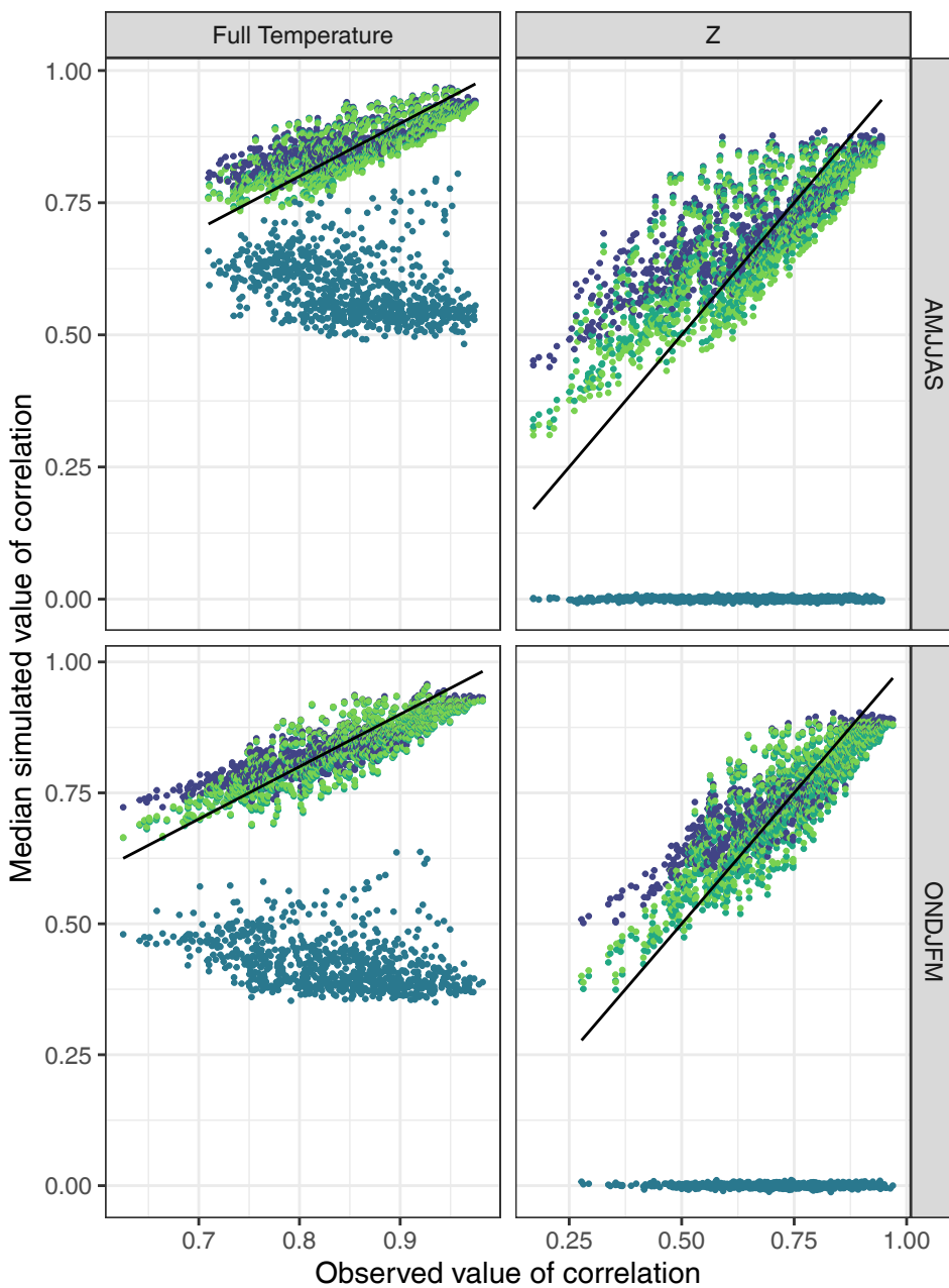
Pairwise correlation between stations
