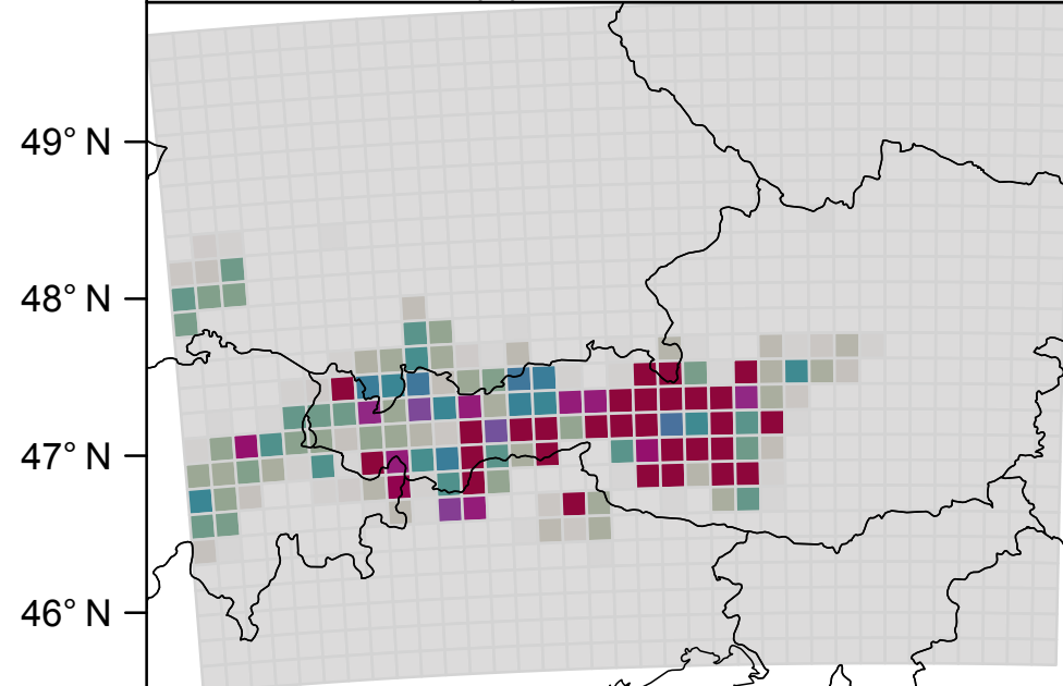
(c) Quantile
