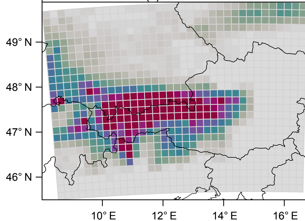
(c) Quantile
