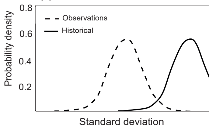
(b) Realization with low Perkins score
