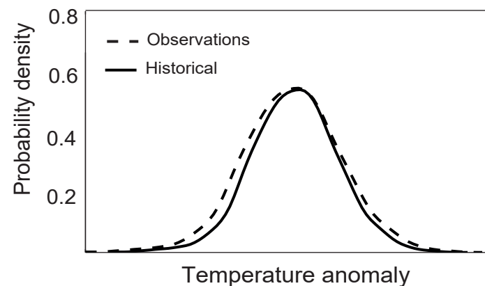
(c) KS test of observed and ensemble distributions = identical
