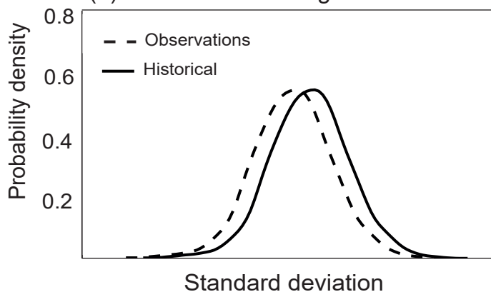
(a) Realization with high Perkins score
