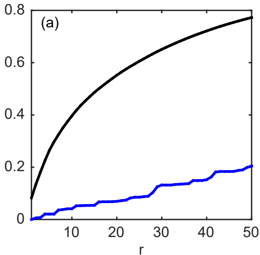
Proportion of total variance
