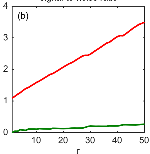
Normalized squared signal-to-noise ratio
