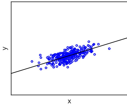
(b) Optimal transformation
