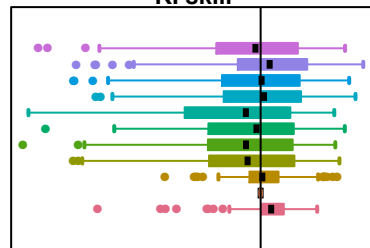
RI skill
