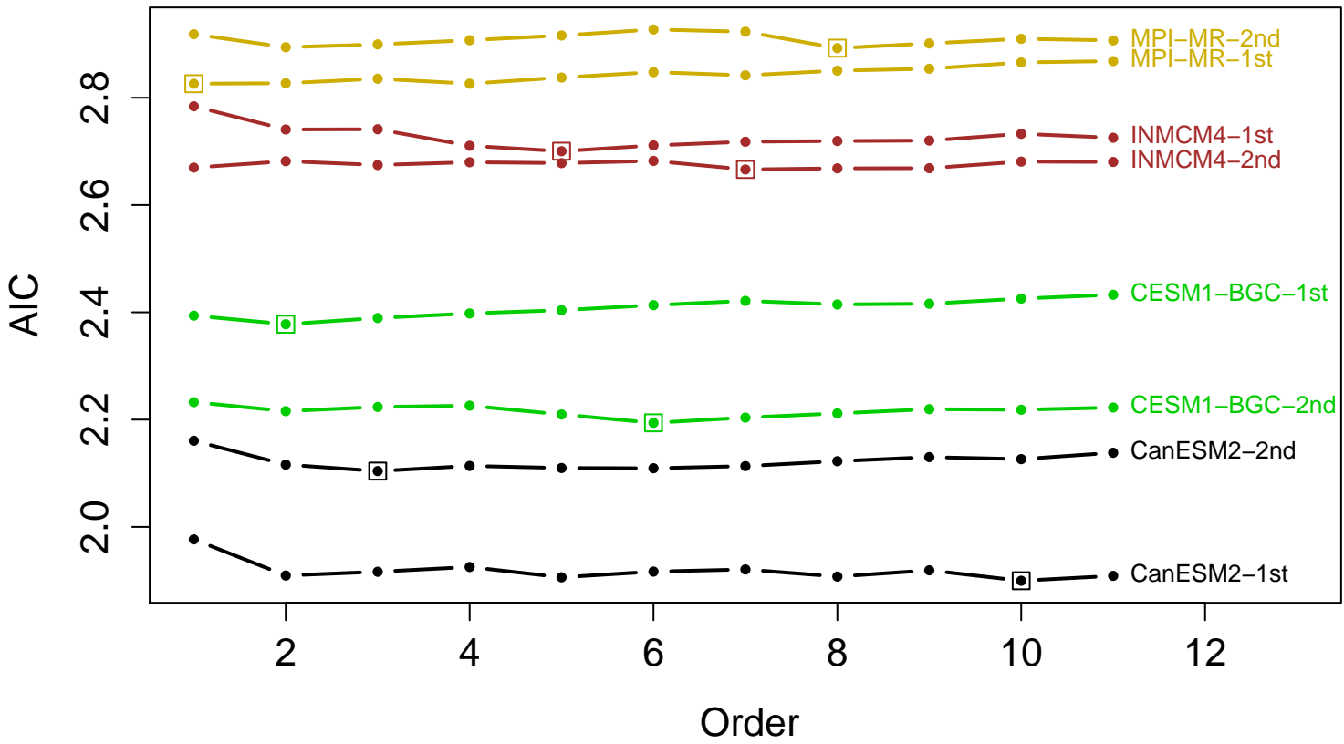
AIC for autoregressive models of amoc
