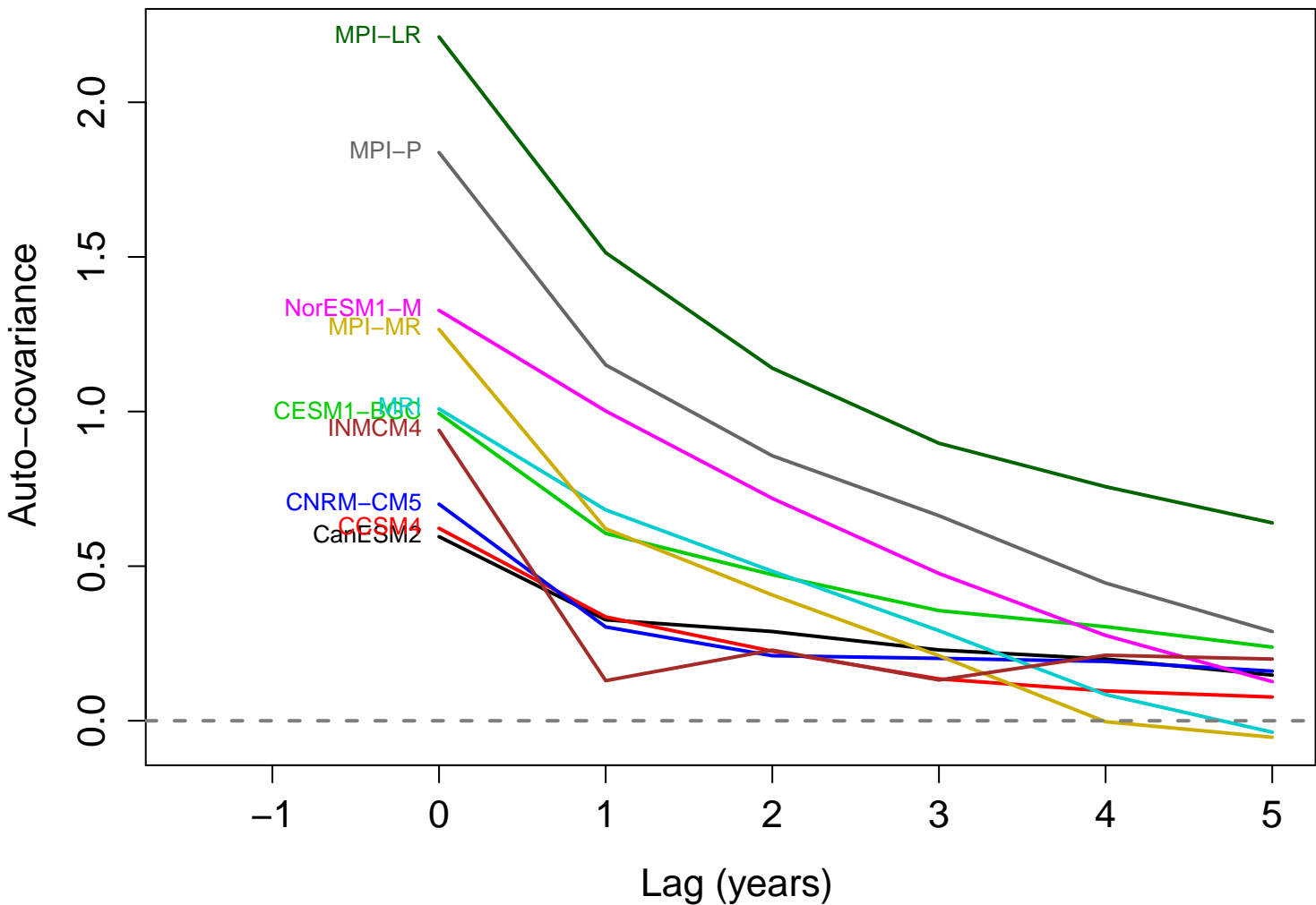
Auto-covariance function of AMOC index in CMIP5 models
