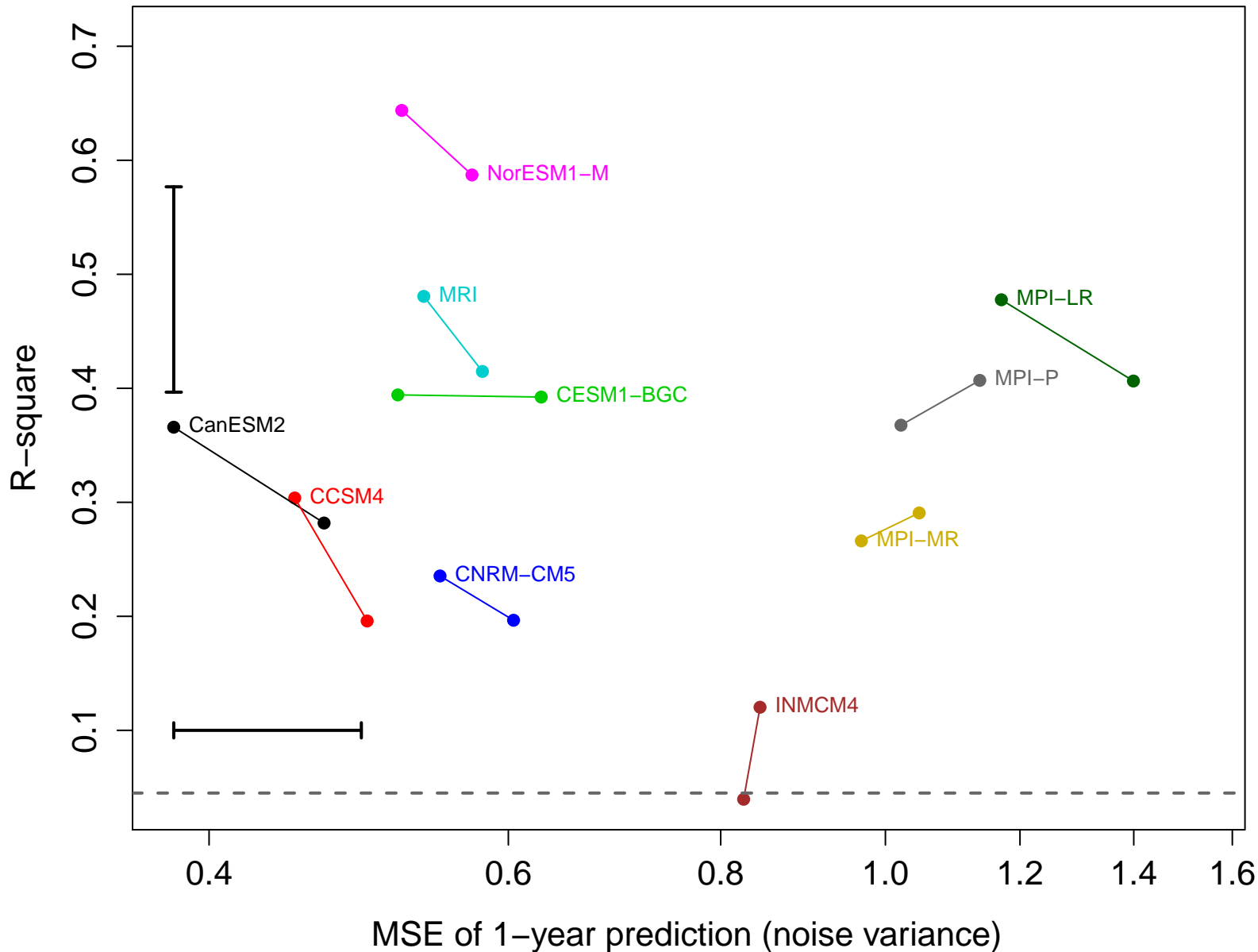
Predictability–noise variance plot of AMOC time series estimated by fitting 250 years to AR(5) model
