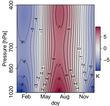
(b) f_2(\text{doy}) + f_3(p, \text{doy})
