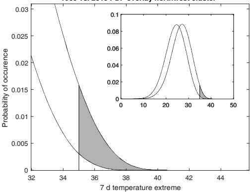
Nonstationary GEV model for 7 d temperature extremes 1960 vs. 2018 PDF overlay northwest cluster
