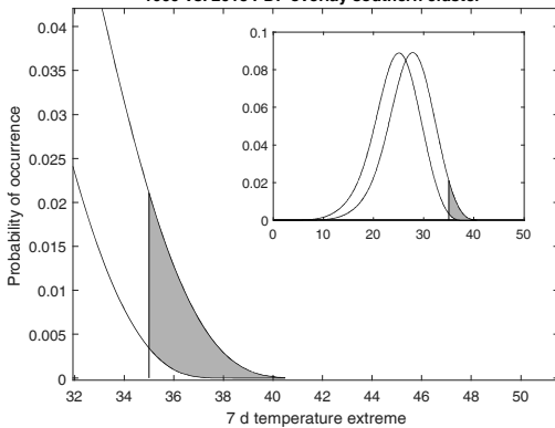
Nonstationary GEV model for 7 d temperature extremes 1960 vs. 2018 PDF overlay southern cluster
