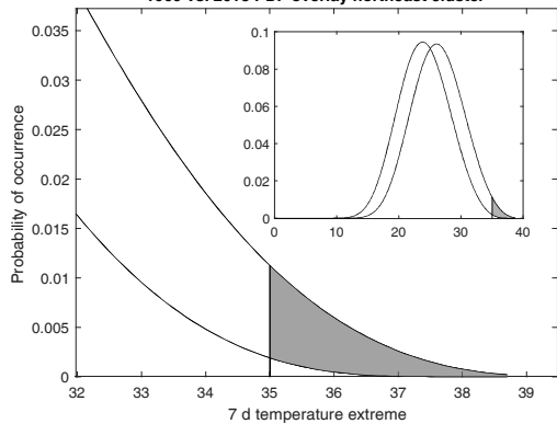
Nonstationary GEV Model for 7 d temperature extremes 1960 vs. 2018 PDF overlay northeast cluster
