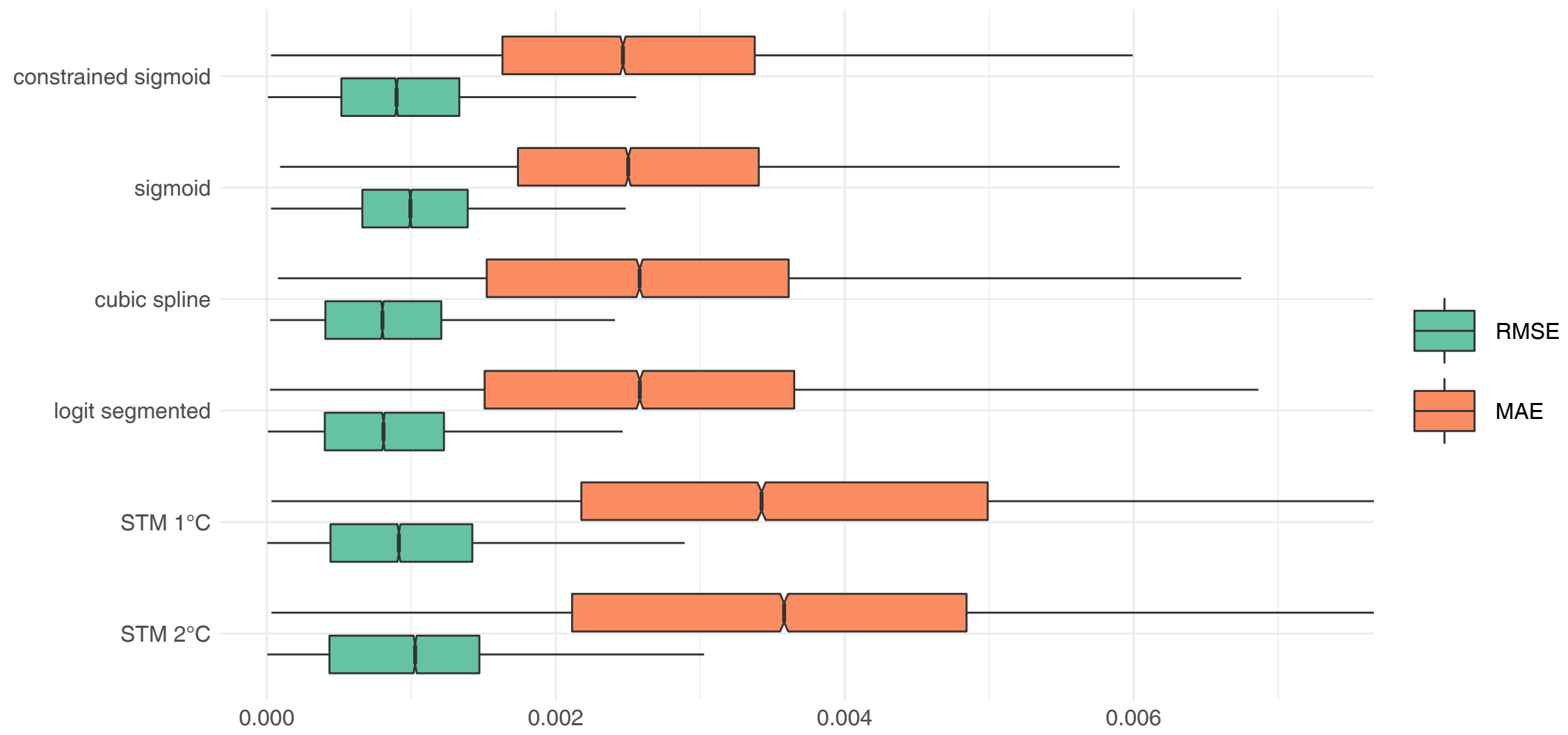
(b) Snowfall (m)
