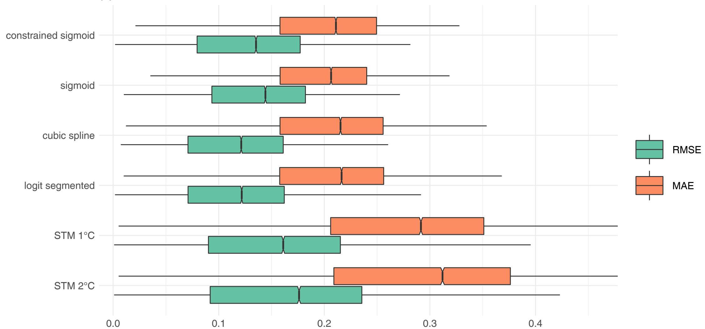
(a) Snow fraction
